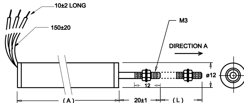
FIGURE1 OUTLINE DIMENSION
